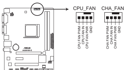
A68HM-E Fan connectors
