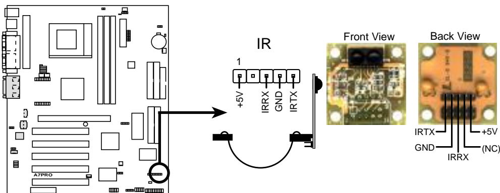
A7PRO Infrared Module Connector
