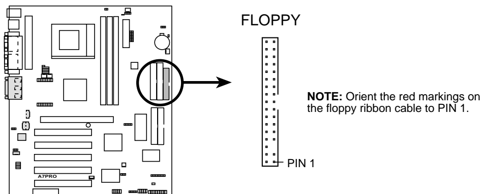
A7PRO Floppy Disk Drive Connector
