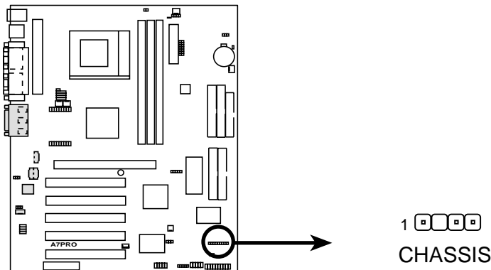
A7PRO Chassis Open Alarm Lead
