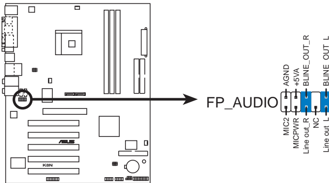
K8N Front panel audio connector
