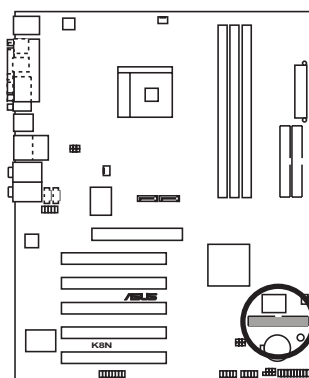
K8N Floppy disk drive connector
