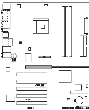
K8N Accelerated Graphics Port (AGP)
