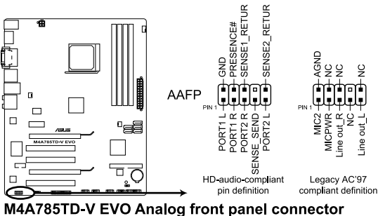
M4A785TD-V EVO Analog front panel connector
