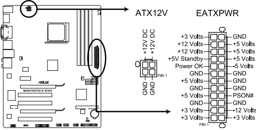
M4A785TD-V EVO ATX power connectors
