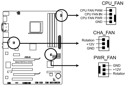
M4A785TD-V EVO fan connectors
