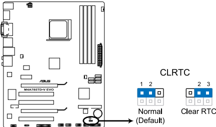
M4A785TD-V EVO Clear RTC RAM
