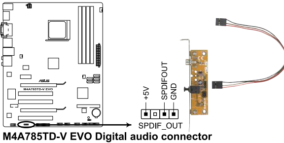
M4A785TD-V EVO Digital audio connector
