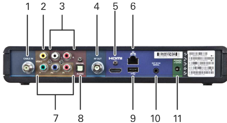
Figure 2: Rear Panel
