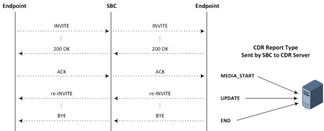
Figure 51-1: CDR Report Types for SBC Media
