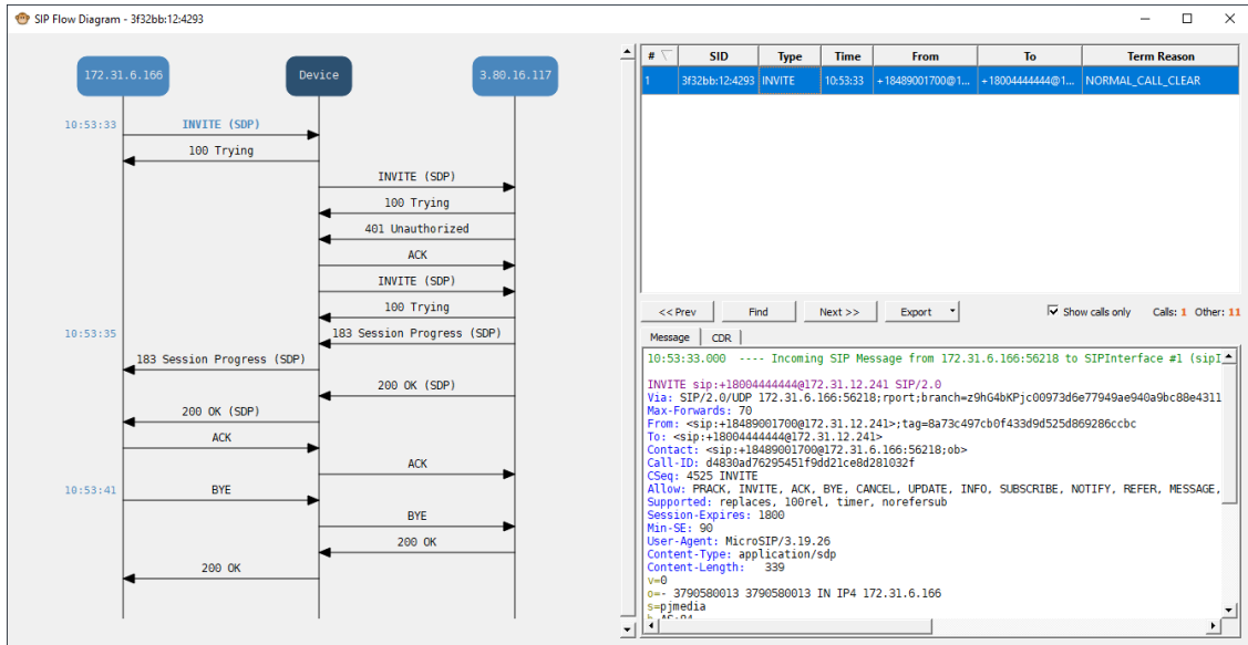
Figure 61-2: Example of SIP Ladder Diagram in Syslog Viewer
