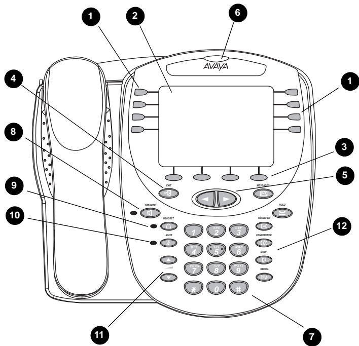
Figure 1: 2420 Telephone Components
