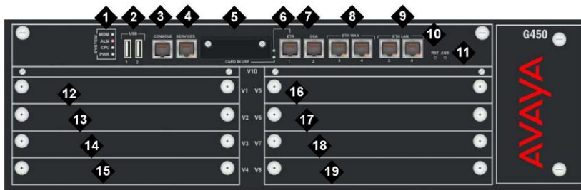
Figure 1: The Branch Gateway G450 1.x Chassis
