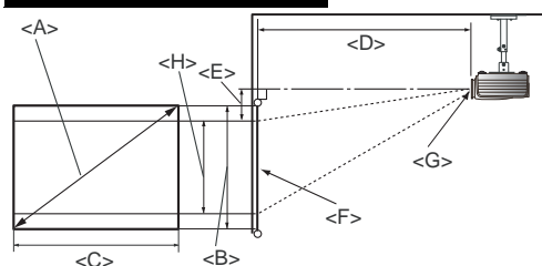
Ceiling Installation
