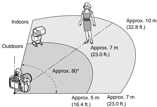
Example of Wireless Flash Set-up
