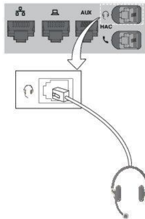
Figure 22: Standard Headset Connection
