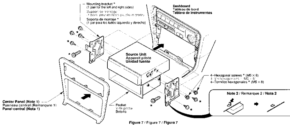
Figure 7 / Figure 7 / Figura 7
