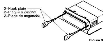
Figure 9 / Figure 9 / Figura 9
