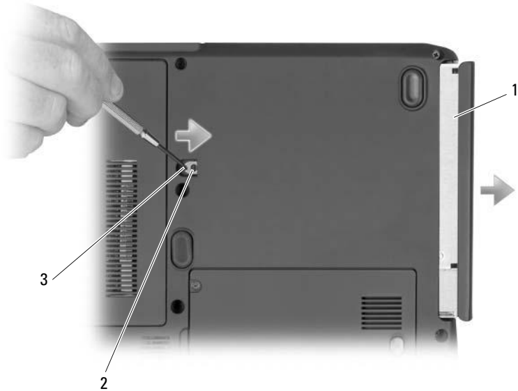
1 optical drive 2 locking screw 3 notch
