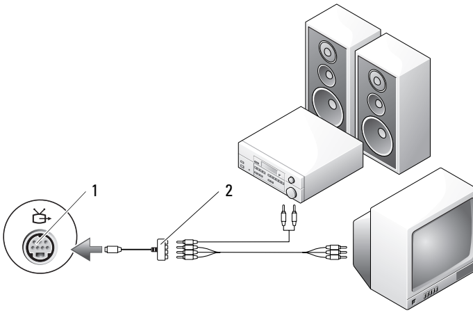
1 S-video TV-out connector 2 component video adapter
