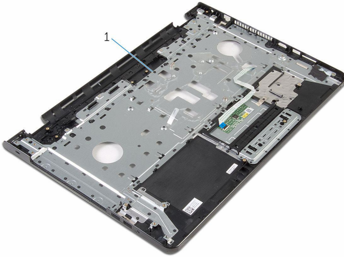
1 palm-rest assembly
