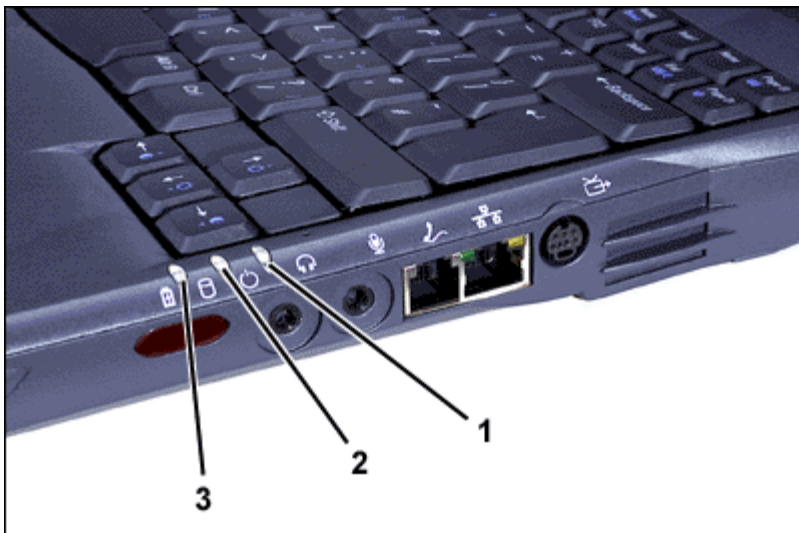
Figure 3. Status Lights
