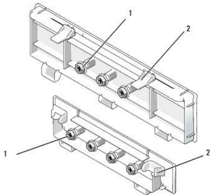
1 shoulder screws 2 plastic drive insert
