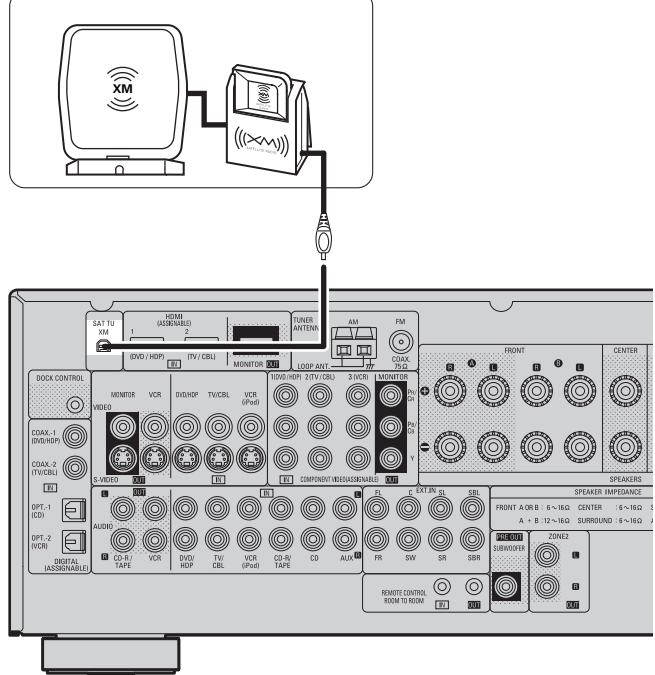
XM Mini-Tuner and Home Dock
