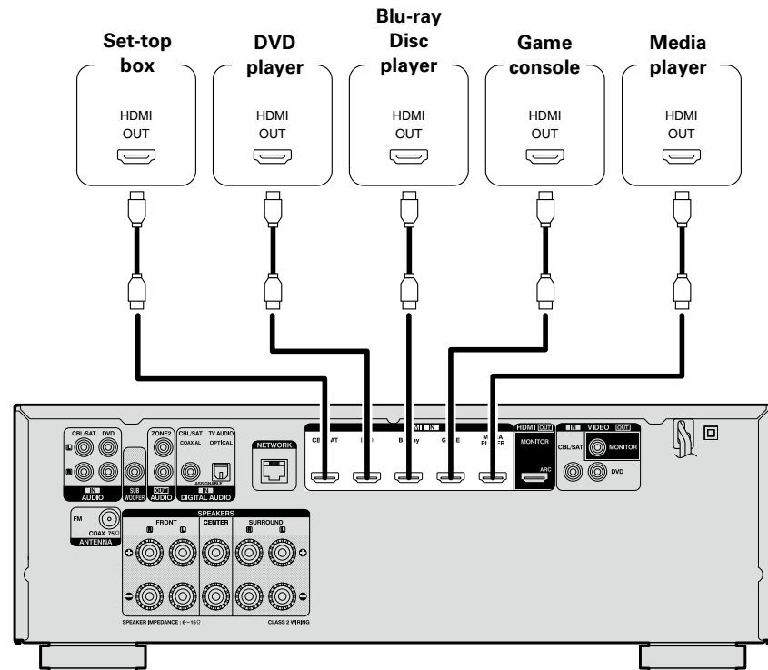
[Rear panel]
