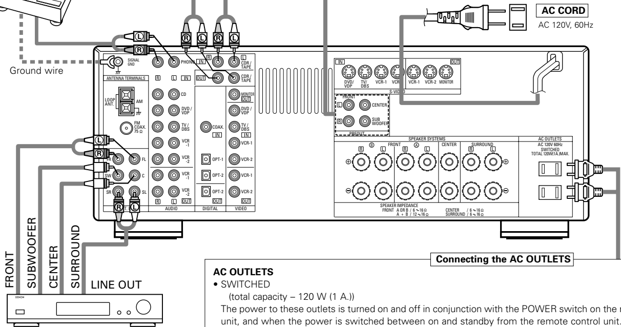
Decoders with 6-channel analog outputs, etc.
