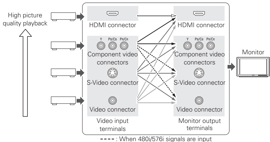
[Flow of video signals inside the AVR-1909]
