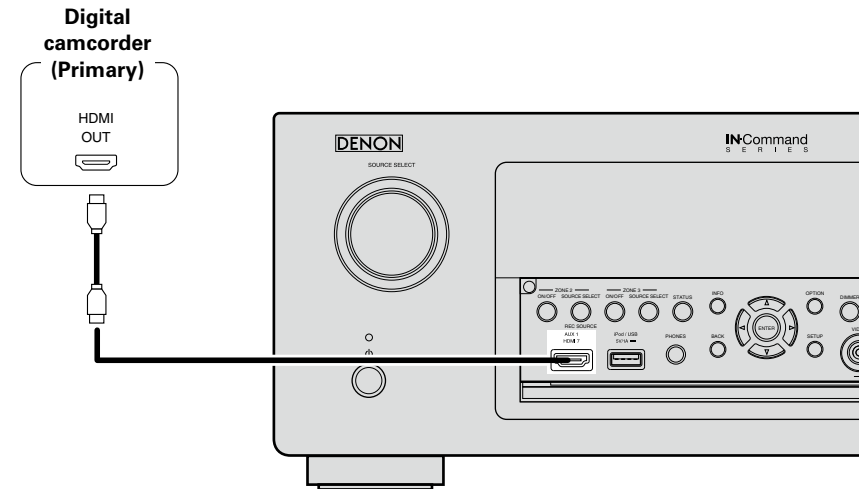
[Front panel]
