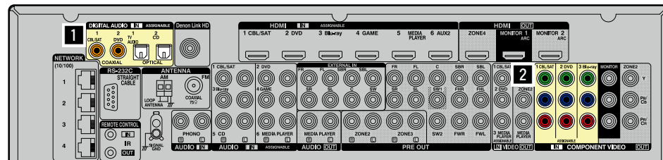
[Rear panel]
