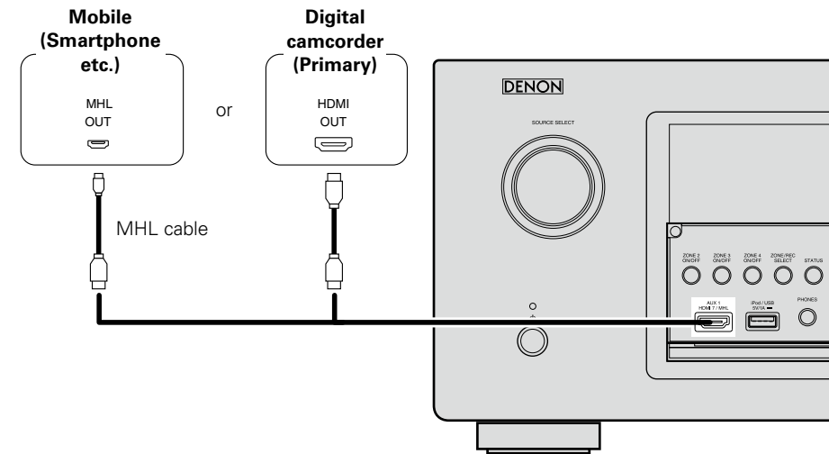
[Front panel]
