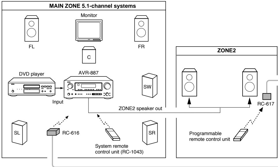
[System configuration and connections example 1] Using this unit's internal amplifier as the ZONE2.
