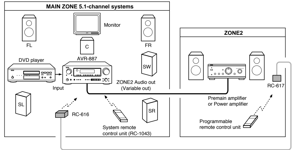
[System configuration and connections example 2] Using external amplifier.
