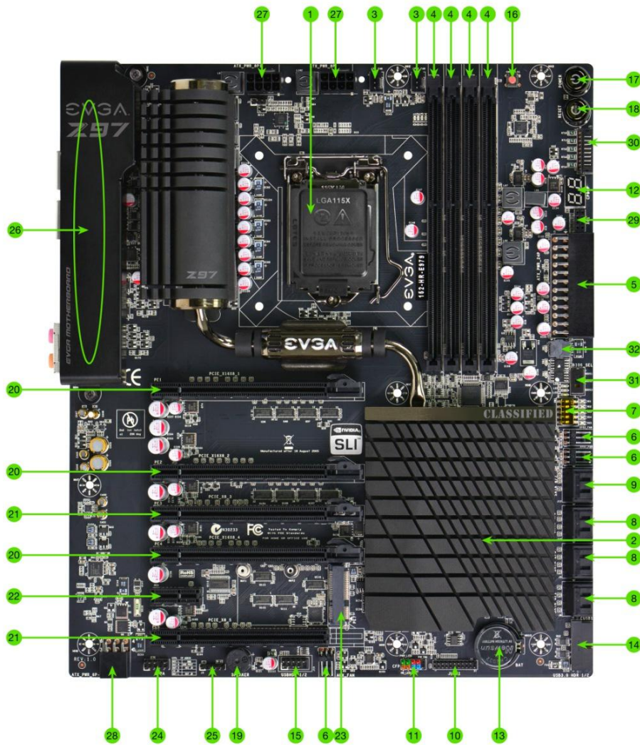
FIGURE 1. Z97 Classified Motherboard Layout
