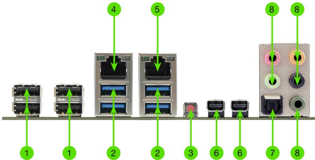
Figure 2. Chassis Rear Panel Connectors
