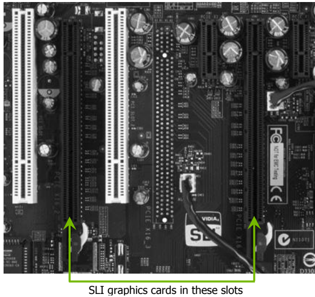
Figure 17. SLI Slots on the Motherboard
