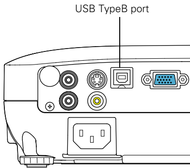
VS200/EX3200
