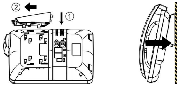
Figure 2 - Wall-mount Installation
