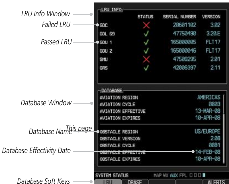
Figure 6-1 System Status
