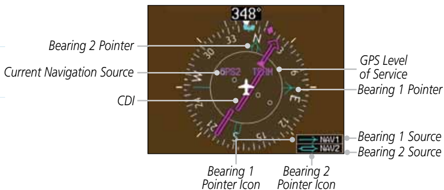
Figure 2-36 HSI with Bearing Information
