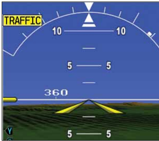
Figure 5-38 Pitch Scale with SVT Enabled
