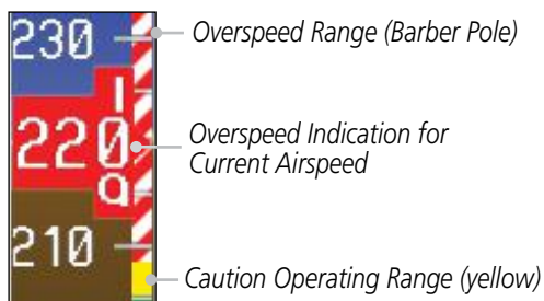
Figure 2-7 Overspeed Indication
