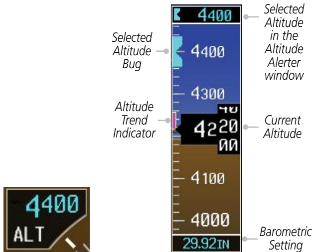
Figure 2-20 Altimeter
