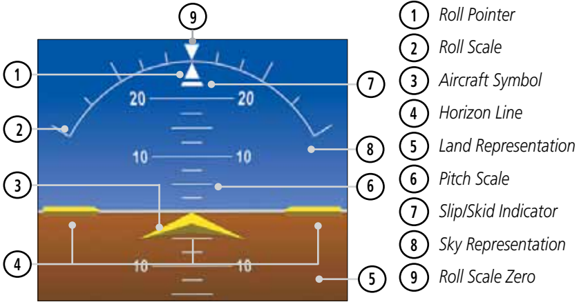
Figure 2-12 Attitude Indicator
