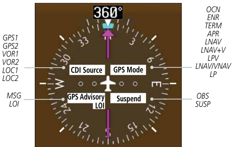
Figure 2-37 PFD HSI Annunciations
