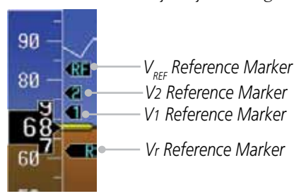
Figure 2-11 Alternate Reference Speeds
