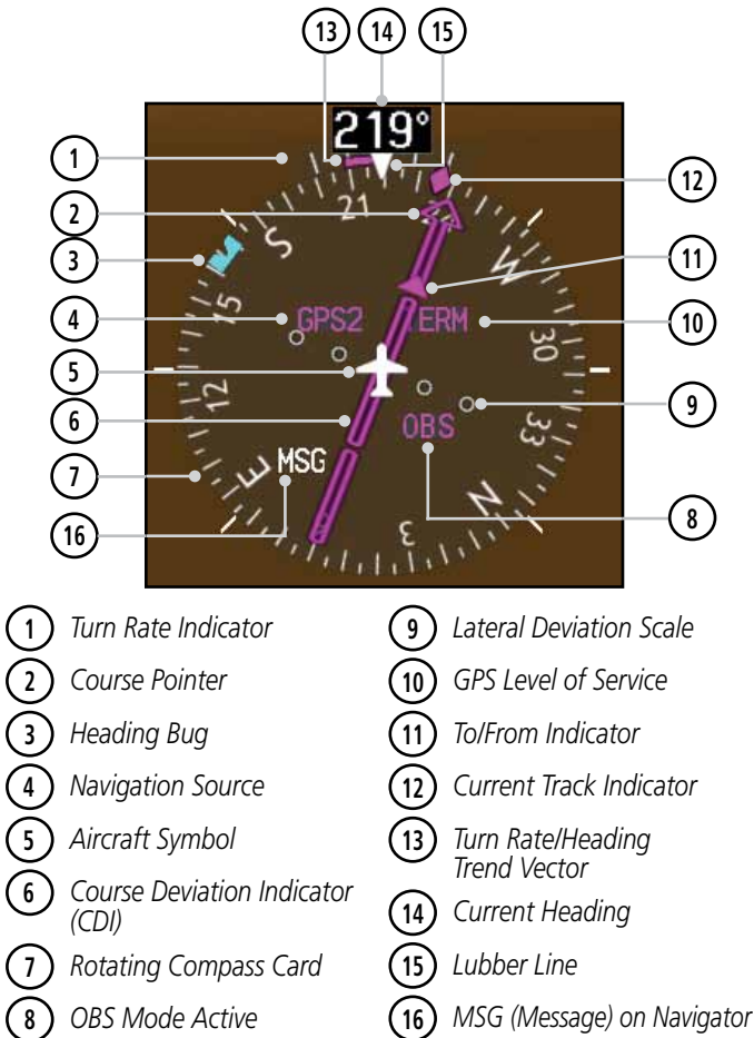
Figure 2-26 Horizontal Situation Indicator (HSI)
