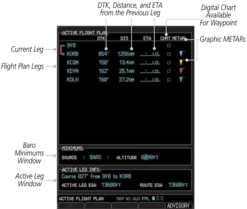
Figure 3-109 Flight Page 1 (Active Flight Plan)
