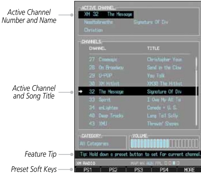
Figure 5-25 XM Radio Presets
