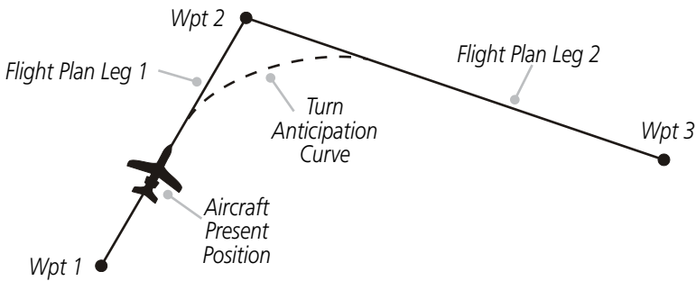
Figure 5-30 GPSS Turn Anticipation
