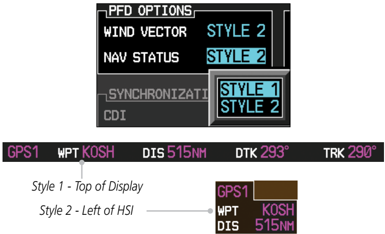
Figure 3-72 Nav Status Style
