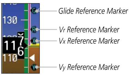
Figure 2-10 Reference Speeds
