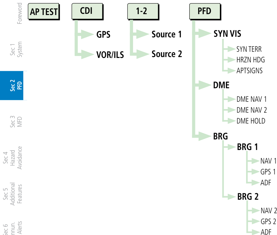
Figure 2-3 PFD Soft Key Diagram
