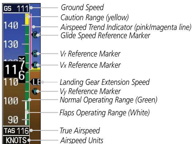
Figure 2-6 Airspeed Tape
