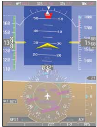
Figure 2-18 Extreme Pitch Indication Nose Up
