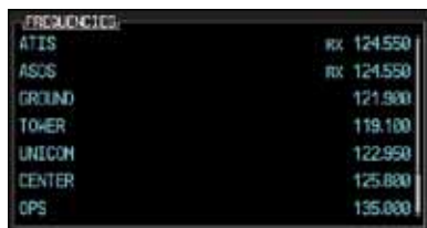
Figure 3-121 Waypoint Frequency Information
