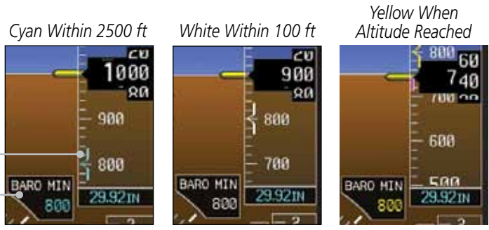
Figure 2-23 Barometric MDA/DH Alerting Visual Annunciations
