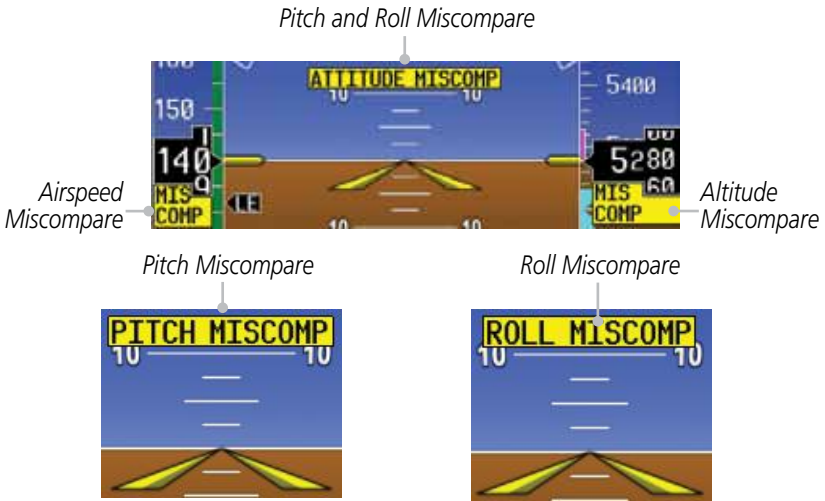
Figure 2-43 Mismatch Annunciations
