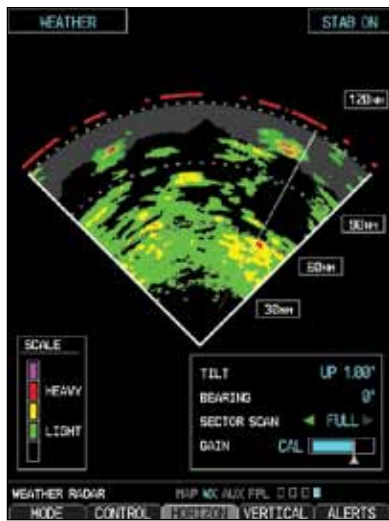
Figure 4-75 Horizontal Scan without WATCHM™ Figure 4-76 Horizontal Scan with WATCHM™
