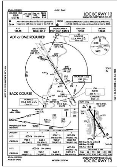
Figure 2-35 Auto-Slewing HSI with Localizer Backcourse Loaded and Shown with the Corresponding Approach Plate
