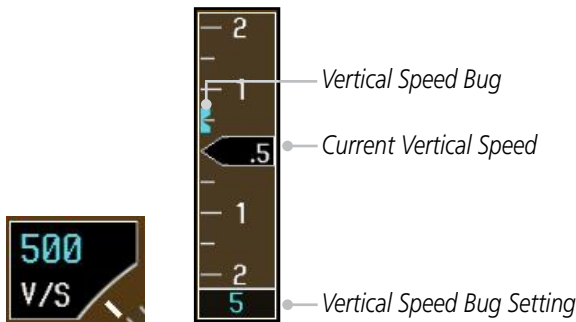
Figure 2-25 Vertical Speed (V/S) Tape and Window
