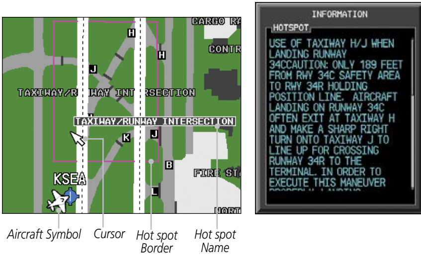
Figure 5-16 SafeTaxi Hot Spot Information
