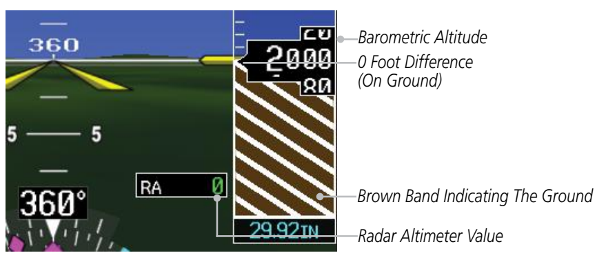
Figure 2-45 Radar Altimeter Display - 0 foot RA Altitude
