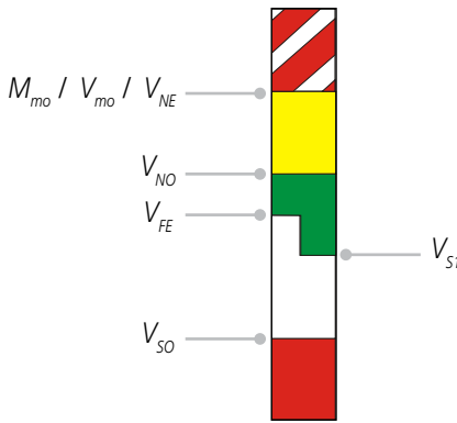
Figure 2-8 Typical Airspeed Tape Markings
