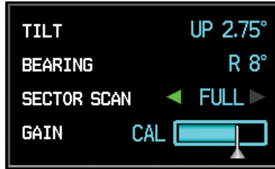
Figure 4-70 Highlight Gain Cal Value
