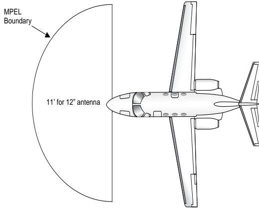
Figure 4-60 MPEL Boundary
