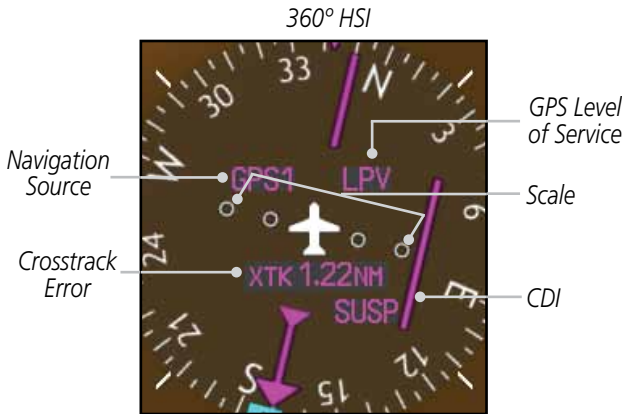
Figure 2-29 Course Deviation Indicator
