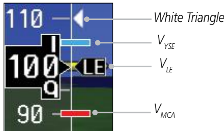
Figure 2-9 Additional Reference Markings
