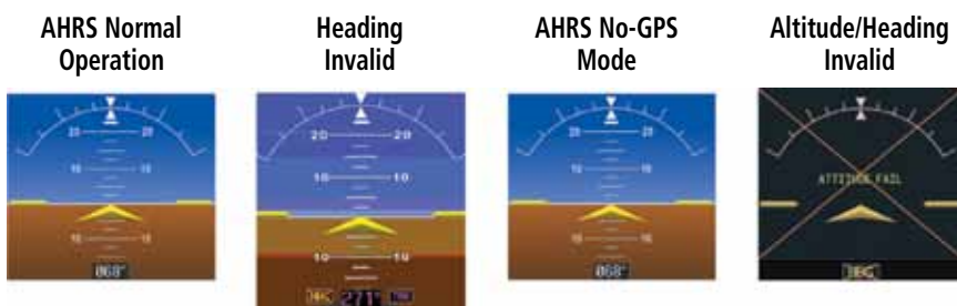
Figure 1-12 AHRS Operation
