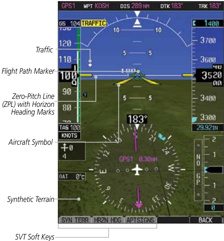
Figure 5-40 SVT on Primary Flight Display
