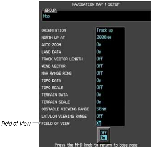
Figure 5-50 Map Setup Items
