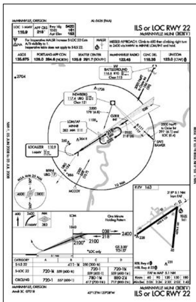
Figure 2-34 Auto-Slewing HSI with ILS Loaded and Shown with the Corresponding Approach Plate
