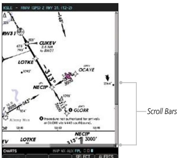
Figure 3-125 Chart Scroll Bars (Charts)
