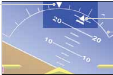
Figure 2-15 Attitude Indicator with a Sky Pointer configuration in a left turn
