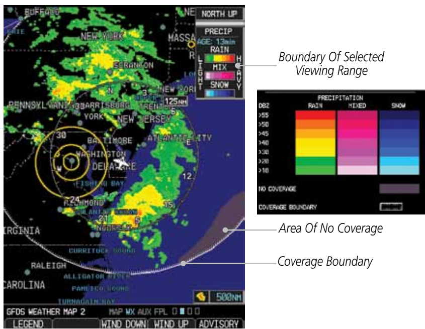
Figure 4-95 GFDS PRECIP Weather Map Display and Legend
