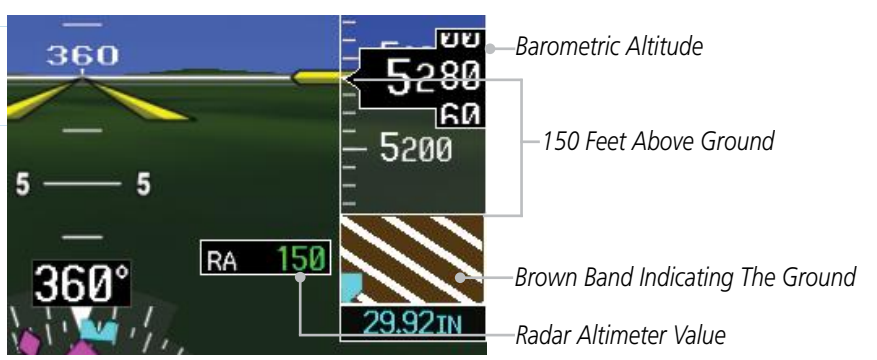
Figure 2-44 Radar Altimeter Display - 150 foot RA Altitude
