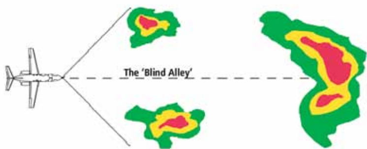
Figure 4-63 The “Blind Alley” Overhead View
