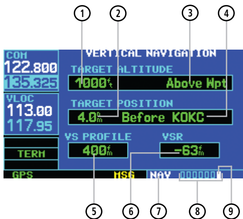
Figure 3-49 Vertical Navigation (VNAV) Page
