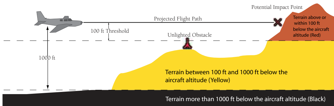
Figure 11-1 Terrain Altitude/Color Correlation
