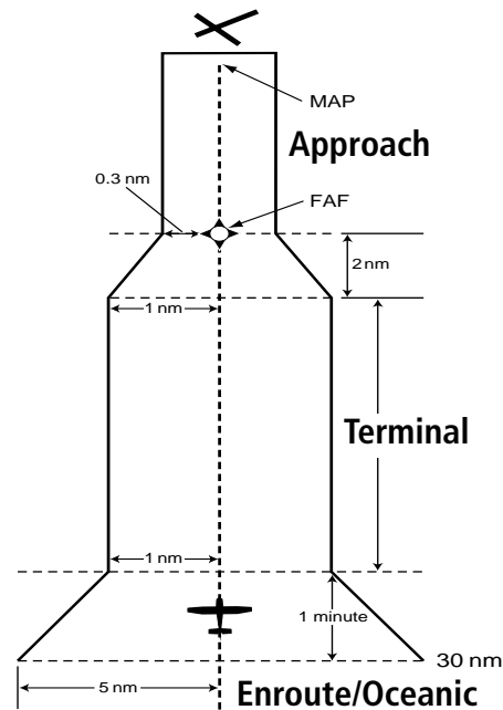
Figure C-7 CDI Scale Transition
