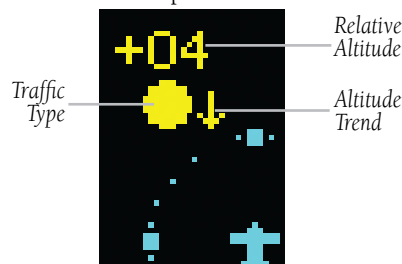
Figure 12-20 Traffic Symbol Components
