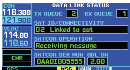
Figure 12-47 Data Link Status Page
