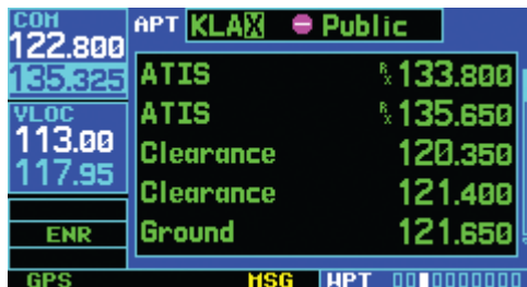
Figure 2-9 Airport Frequencies Page
