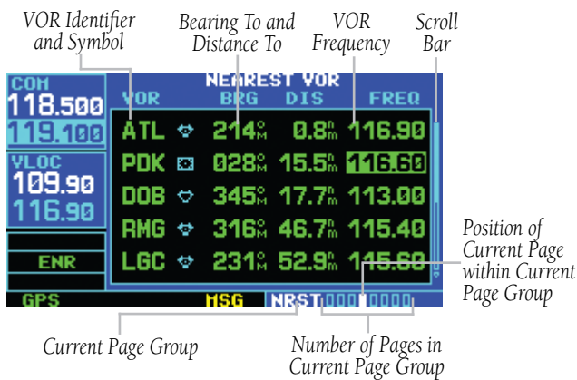
Figure 8-18 Nearest VOR Page
