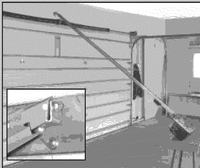
FIG. 2-7 Position assembly.
