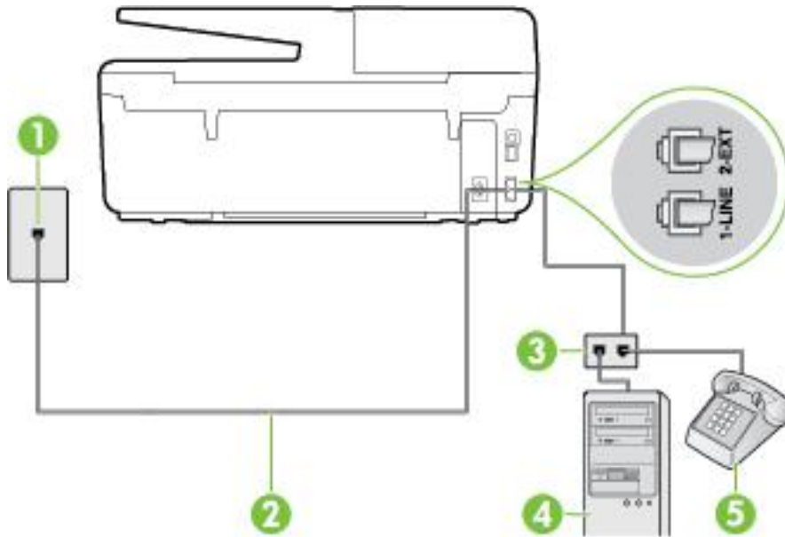
Figure B-9 Back view of the printer
