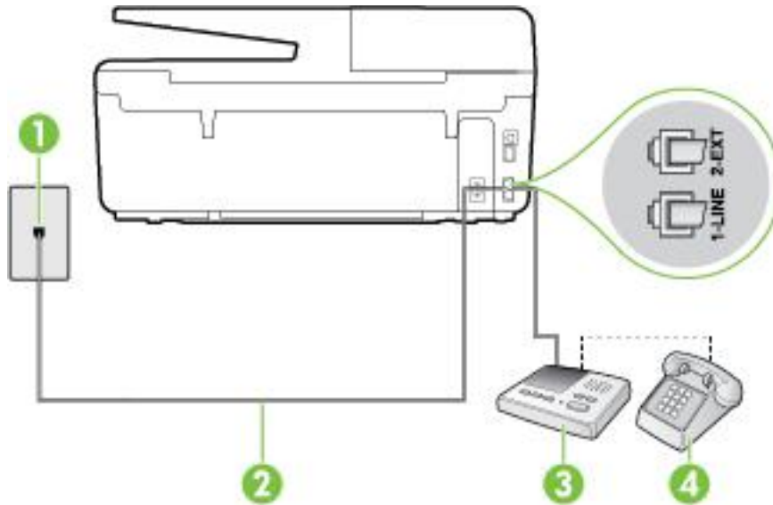
Figure B-11 Back view of the printer
