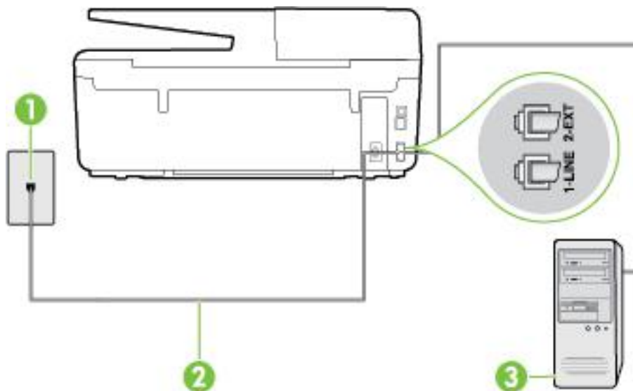
Figure B-6 Back view of the printer
