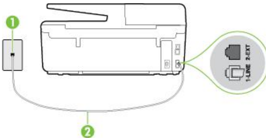
Figure B-1 Back view of the printer
