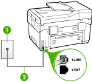
Figure 10-1 Back view of the device
