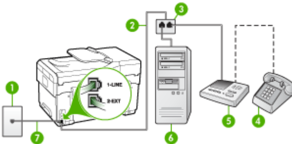
Figure 9-11 Back view of the device
