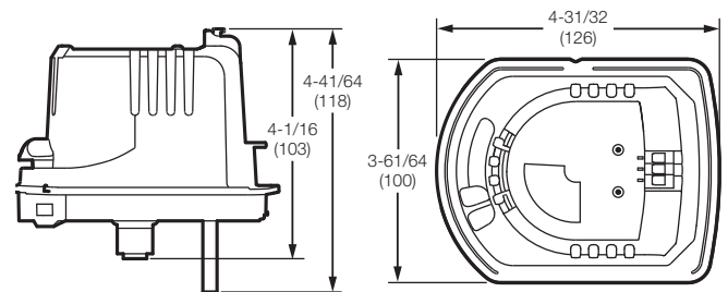
Fig. 1. Dimensional Details.
