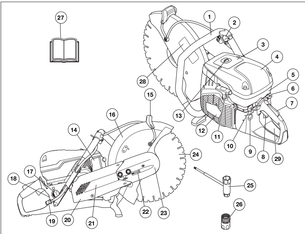
What is what on the power cutter - K970 II?
