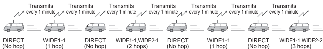
Figure 6-2 Example of path switchover operation of Proportional Pathing (when the packet path is set to WIDE1-1, WIDE2-2)
