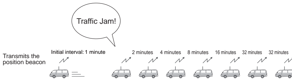
Figure 6-1 Decay Algorithm
