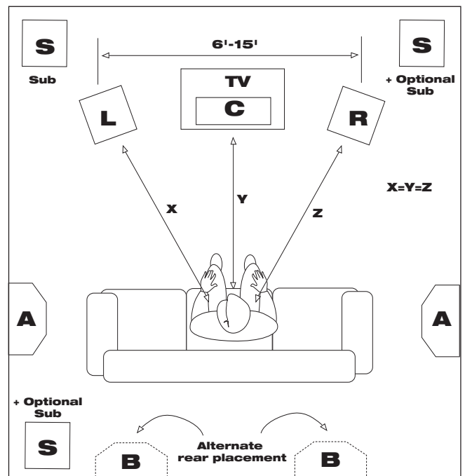
SURROUND LCR AND REARS
