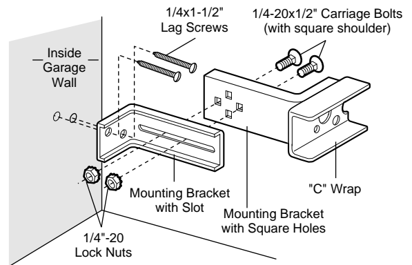
Figure 4 Garage WALL Installation
