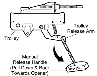
Lockout position
