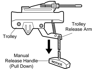
Manual disconnect position
