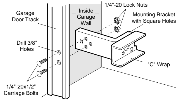
Figure 3 Garage DOOR Track Installation
