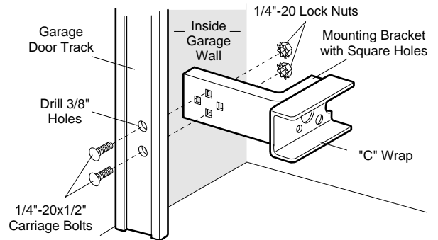
Figure 4 Garage WALL Installation
