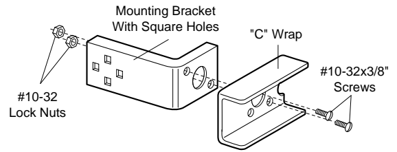
Figure 3 Garage DOOR Track Installation
