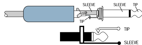
Figure C: Tip-Sleeve (TS) Mono Connector
