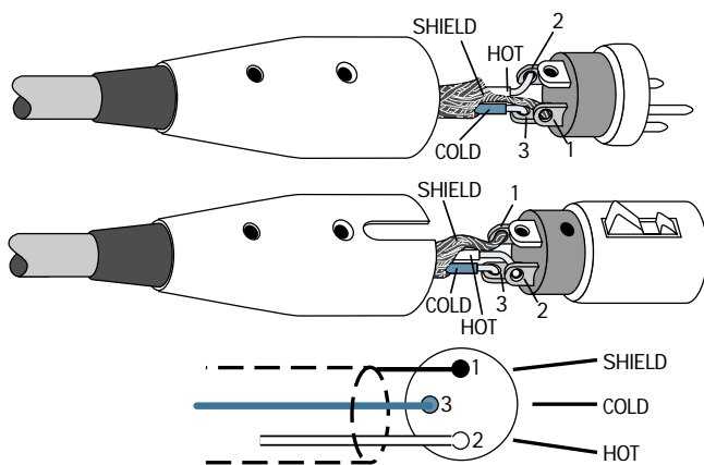
Figure A: XLR Connectors
