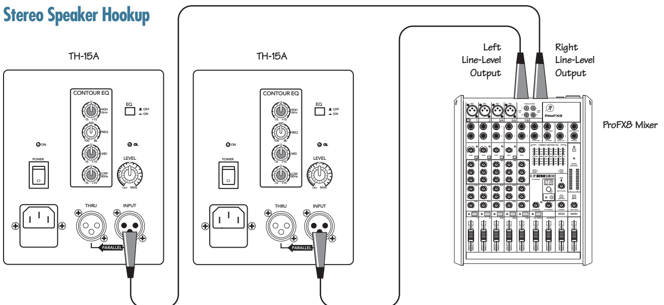
The left and right line-level outputs from a mixer feed the inputs of two Mackie TH-15A Powered Loudspeakers.
