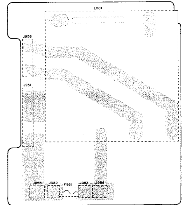
P951 Transformer/Fuse
