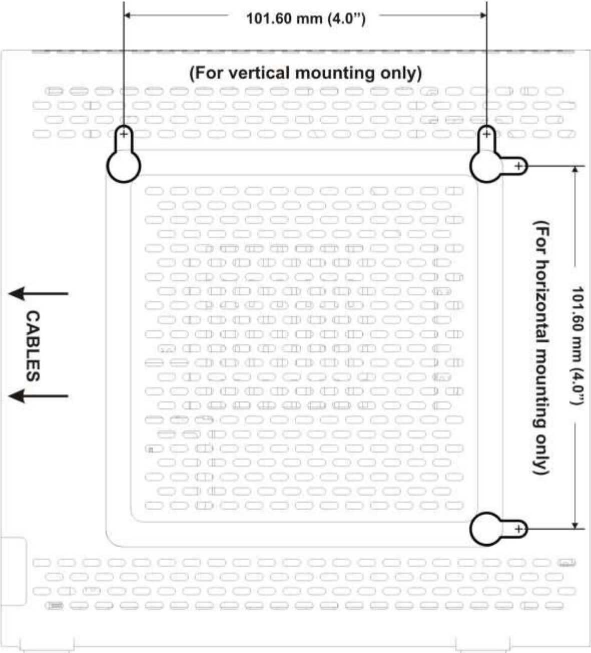
Figure 5: Sample SBG6580 Wall Mounting Template
