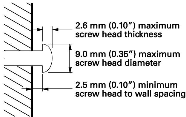
Figure 4: Wall Mount-Screw Head Dimensions
