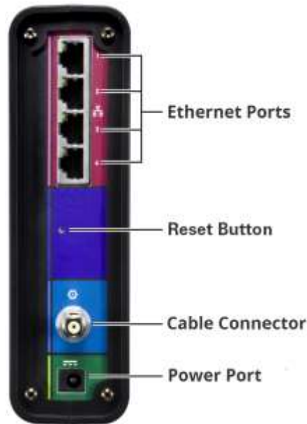
Figure 2: SBG6580 Rear View
