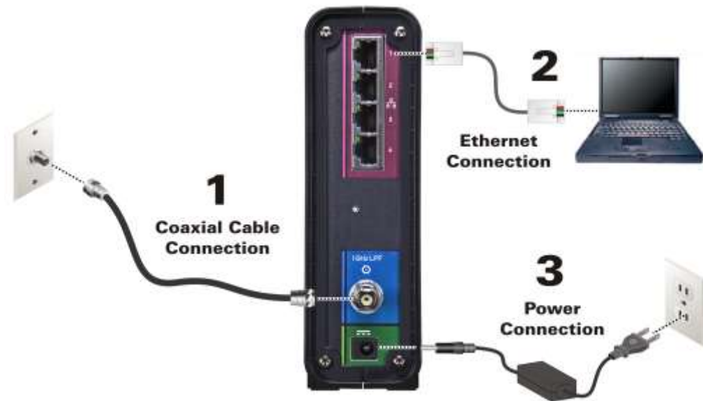
Figure 3: SBG6580 Connection Diagram
