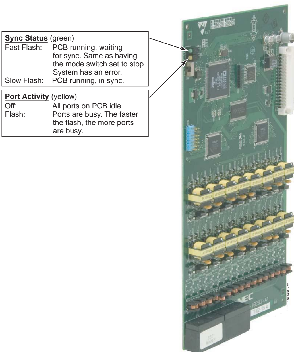
Figure 35: Digital Station (ESIU), Analog Station (SLIU), and Analog Line (COIU) Card LEDs
