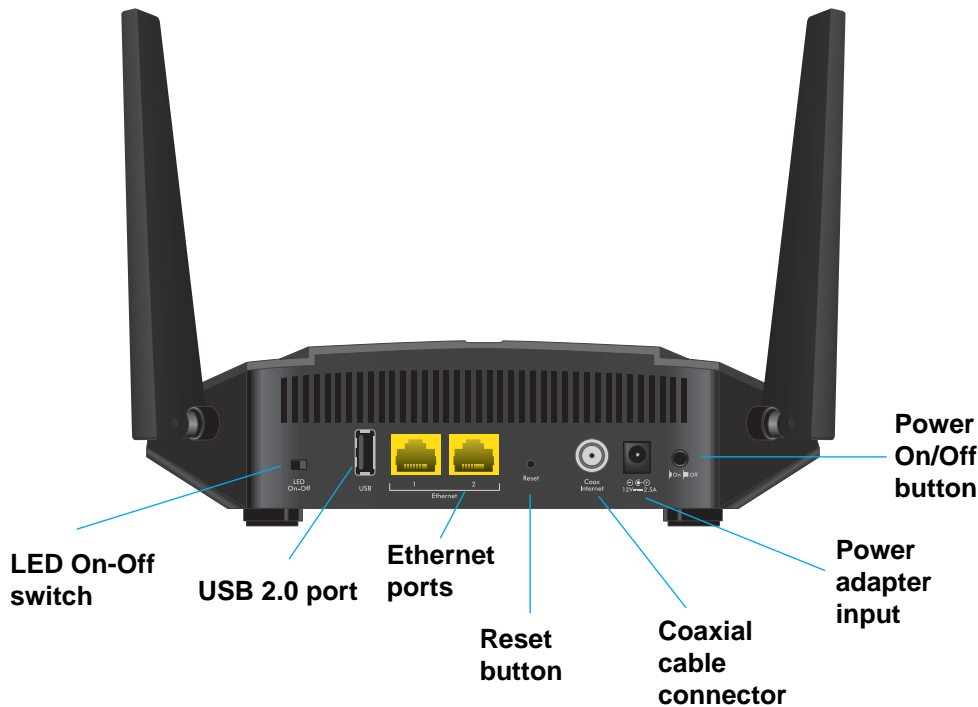
Figure 3. Modem router rear panel
