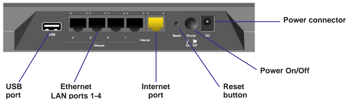
Figure 3. Router, rear view
