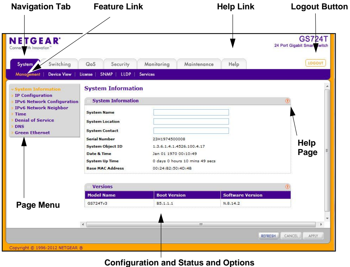
Figure 4. Administrative Page Layout
