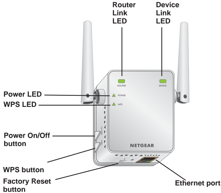
Figure 1. Front panel
